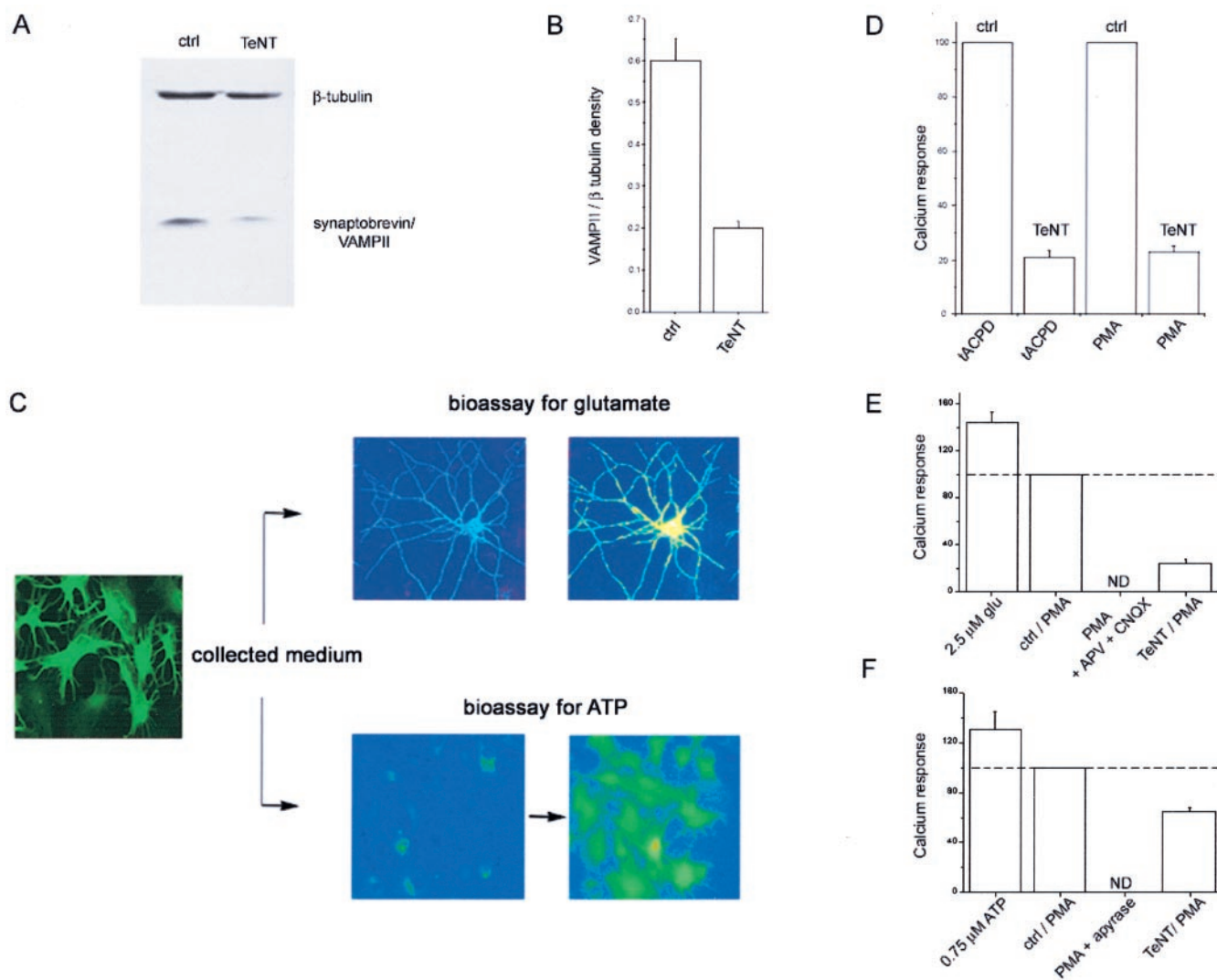
FIG. 5. TeNT differently affects ATP and glutamate release from astrocytes. A , Western blot analysis of control and TeNT-intoxicated cultured rat astrocytes shows that synaptobrevin/VAMP11 is massively cleaved by the clostridial toxin. \beta -tubulin staining is shown as a standard. B , quantitative analysis of synaptobrevin/VAMP11 content in control and intoxicated cultures. Synaptobrevin/VAMP11 immunoreactivity is normalized to \beta -tubulin staining. C , schematic representation of glutamate and ATP measurements in medium conditioned by the same astrocyte monolayer. Aliquots of conditioned medium collected before and after TeNT intoxication were split into two parts and tested in parallel on glutamate reporter neurons and ATP reporter cells. D , quantitative analysis of the glutamate released by t-ACPD- or PMA-treated astrocyte monolayers before and after 24-h TeNT intoxication (t-ACPD: 21 \pm 2.6\% residual [Ca^{2+}]_i response after TeNT, n = 9 ; PMA: 23 \pm 2.2\% residual [Ca^{2+}]_i response after TeNT, n = 11 ). E and F , quantitative analysis of TeNT sensitivity of glutamate ( E , 24 \pm 3.5 residual [Ca^{2+}]_i response after TeNT, n = 24 ) and ATP release ( F , 65 \pm 3\% residual [Ca^{2+}]_i response after TeNT, n = 17 ) from the same intoxicated astrocyte culture. The histograms in D , E , and F show percent changes ( \pm S.E.) normalized to the [Ca^{2+}]_i responses induced by medium conditioned by astrocyte monolayers before TeNT intoxication. N.D. , not detectable.
